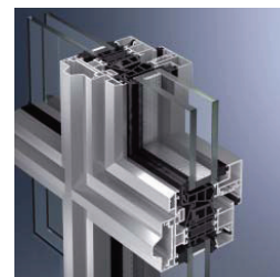
Schüco AWS 70 WF.HI con tapetas Schüco AWS 70 WF.HI with cover cap
